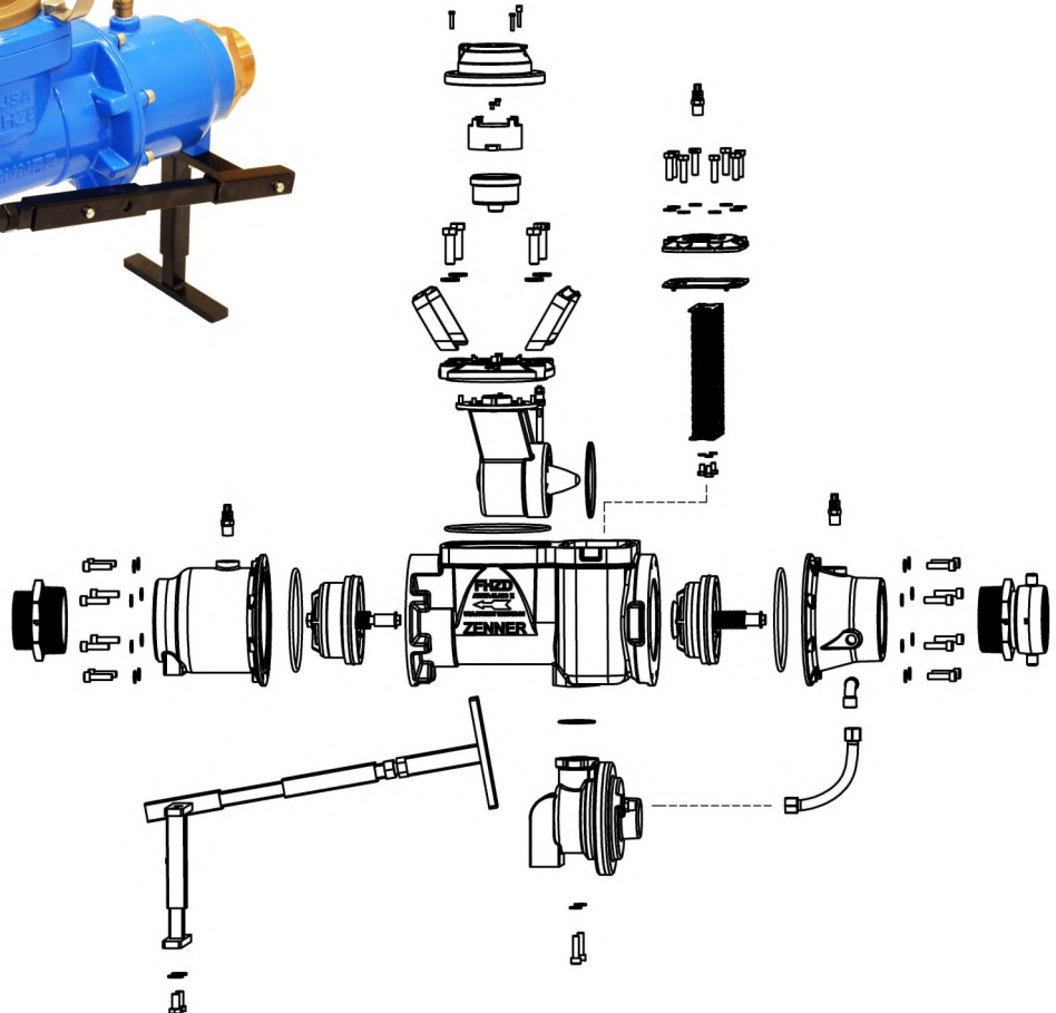
FHZD30S**-RP Configured with optional 2-1/2" ZHGV250 Hydrant Gate Valve (Eddy Valve)
